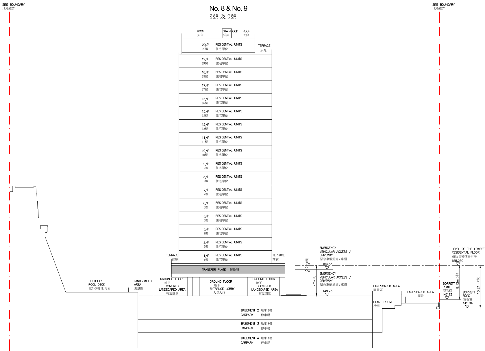
橫截面圖A-A CROSS SECTION PLAN A-A
