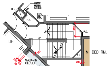
PART PLAN AT 29/F 29樓 局部平面圖
