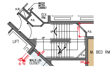
PART PLAN AT 30/F-41/F 30樓至41樓 局部平面圖
