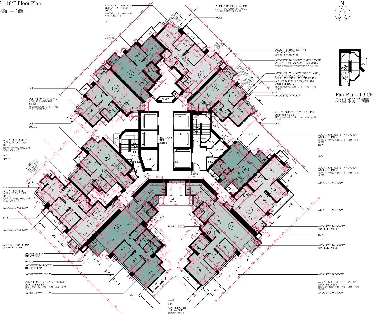
Tower 8 30/F - 33/F, 35/F -43/F and 45/F - 46/F Floor Plan
