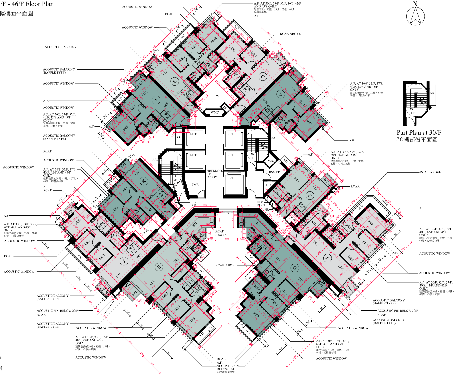
Part Plan at 30/F 30樓部份平面圖
