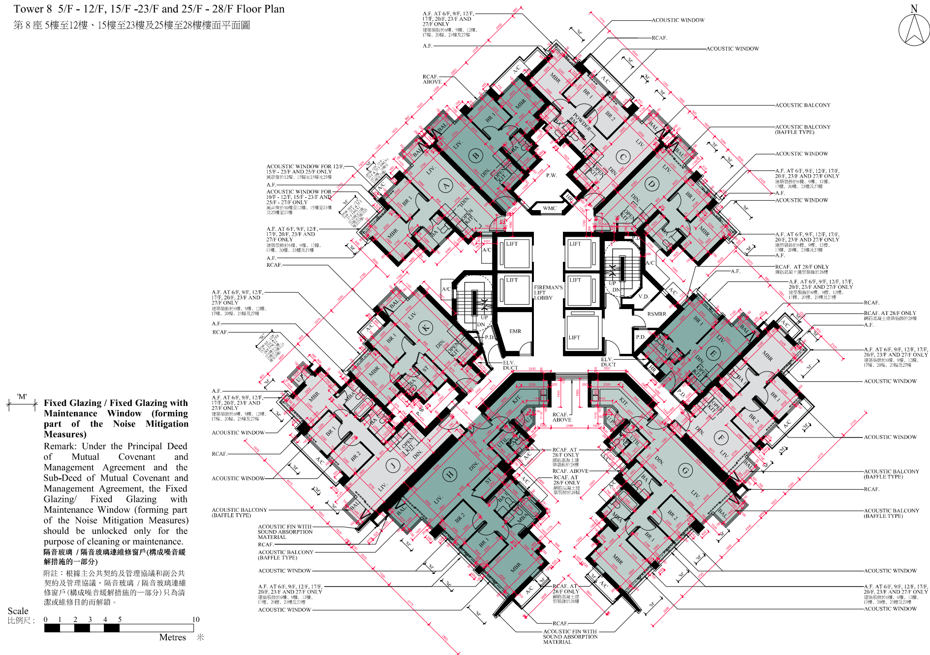
Tower 8 5/F - 12/F, 15/F - 23/F and 25/F - 28/F Floor Plan
