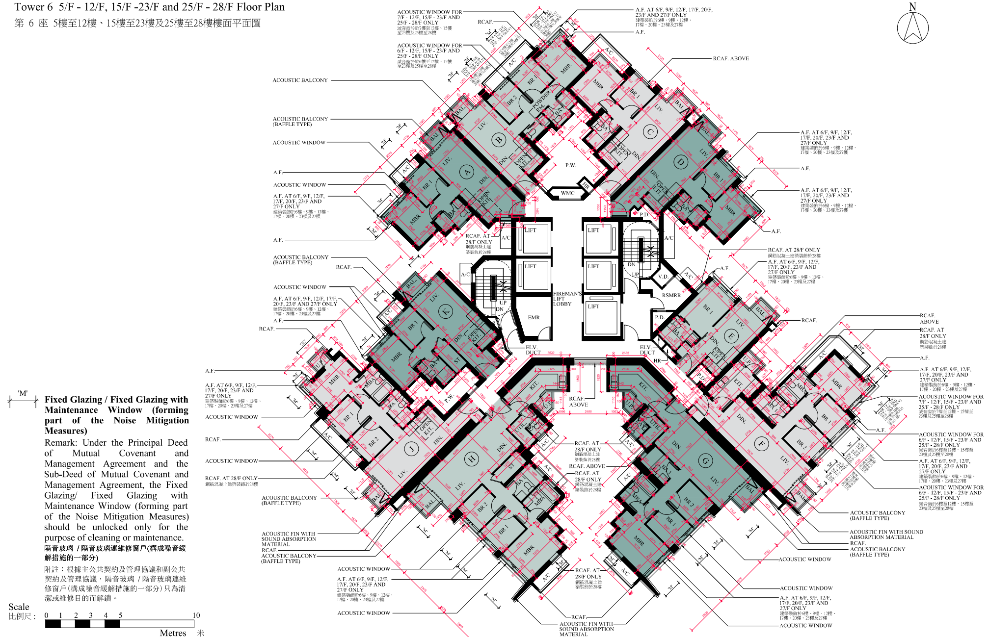
Tower 6 5/F - 12/F, 15/F - 23/F and 25/F - 28/F Floor Plan
