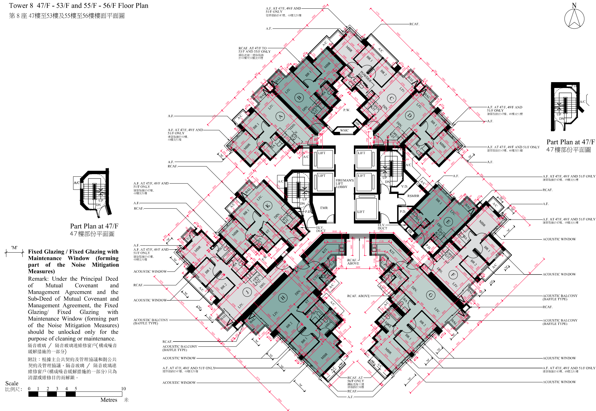
Tower 8 47/F - 53/F and 55/F - 56/F Floor Plan
