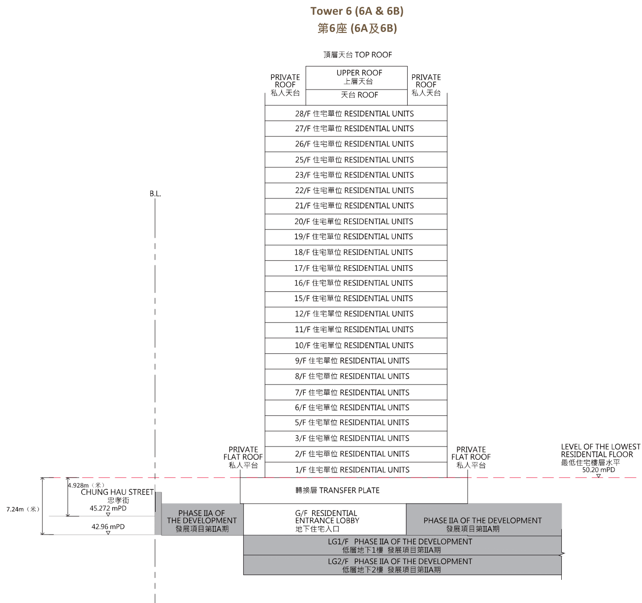
Cross-section Plan B-B 橫截面圖B-B
