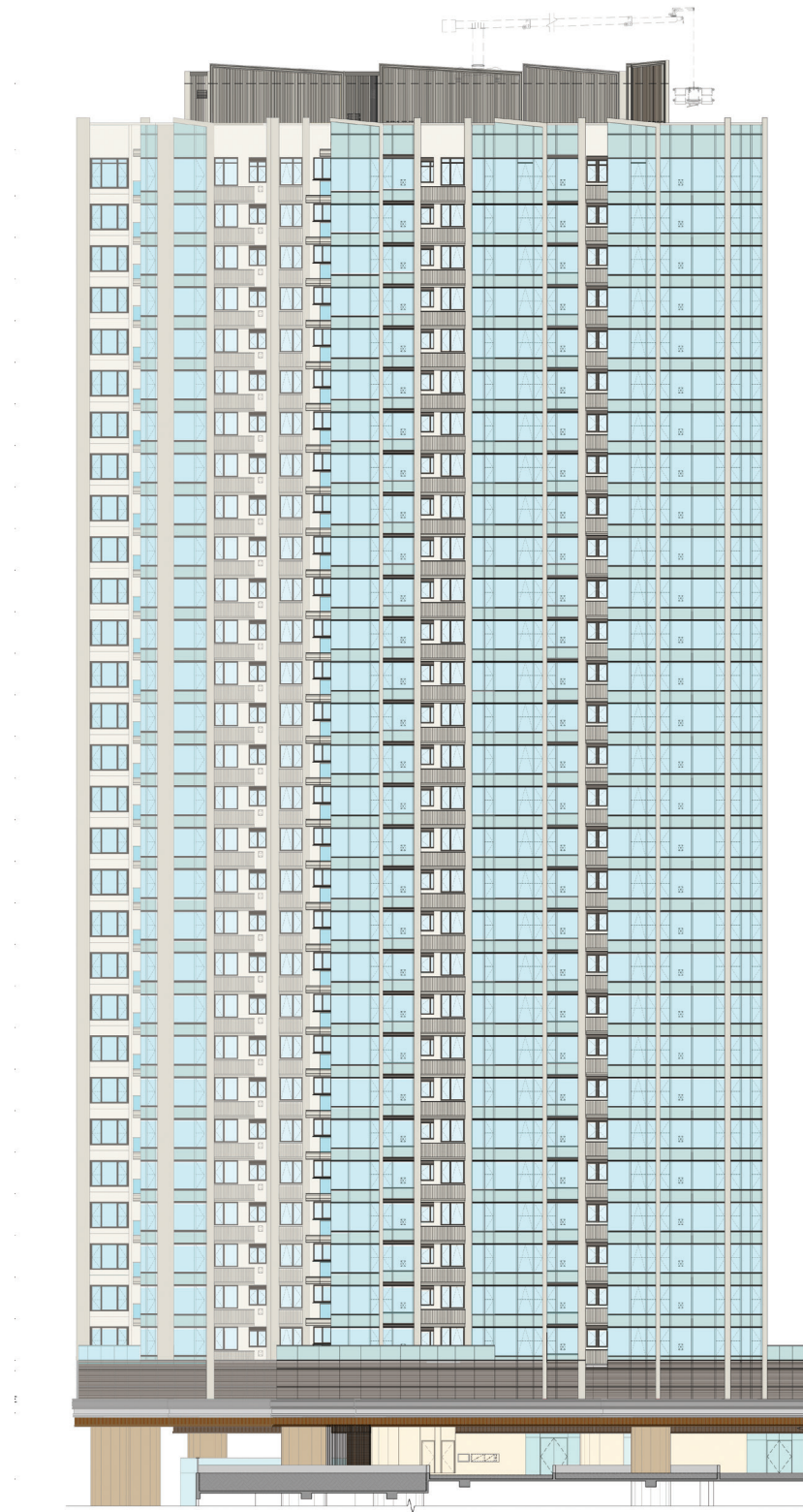
立面圖3 Elevation Plan 3
