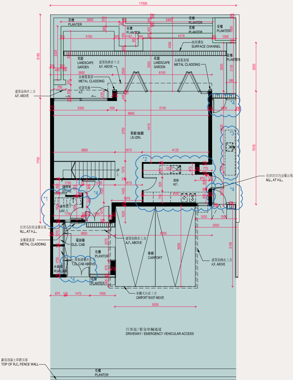
HOUSE NO. 52B, HOUSE NO. 52C and HOUSE NO. 52D GROUND FLOOR PLAN 52B號洋房、52C號洋房及52D號洋房地下平面圖 Latest "As -is" Layout Plan 現狀間隔平面圖
