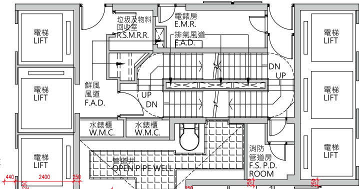
Tower 3 (3A & 3B) 22/F Part Plan
