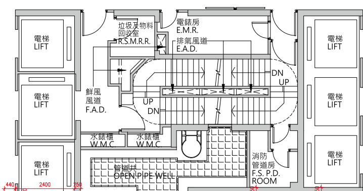
Tower 3 (3A & 3B) 48/F Part Plan
