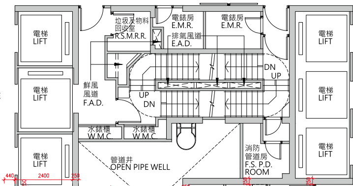
Tower 3 (3A & 3B) 47/F Part Plan
