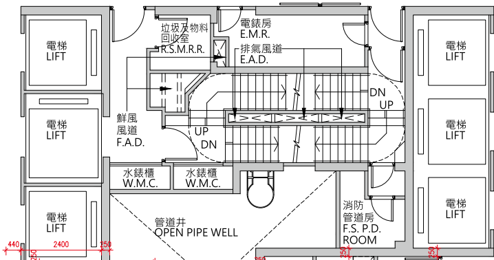
Tower 3 (3A & 3B) 20/F Part Plan
