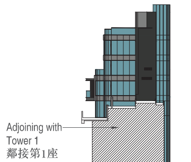
MANSION 1 ELEVATION 4 MANSION 1 立面4
