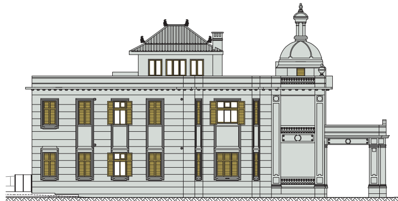
⑨ LEFT ELEVATION (NORTH-WEST) 左立面 (西北立面)
