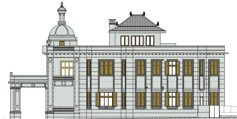
⑩ RIGHT ELEVATION (SOUTH-EAST) 右立面 (東南立面)
