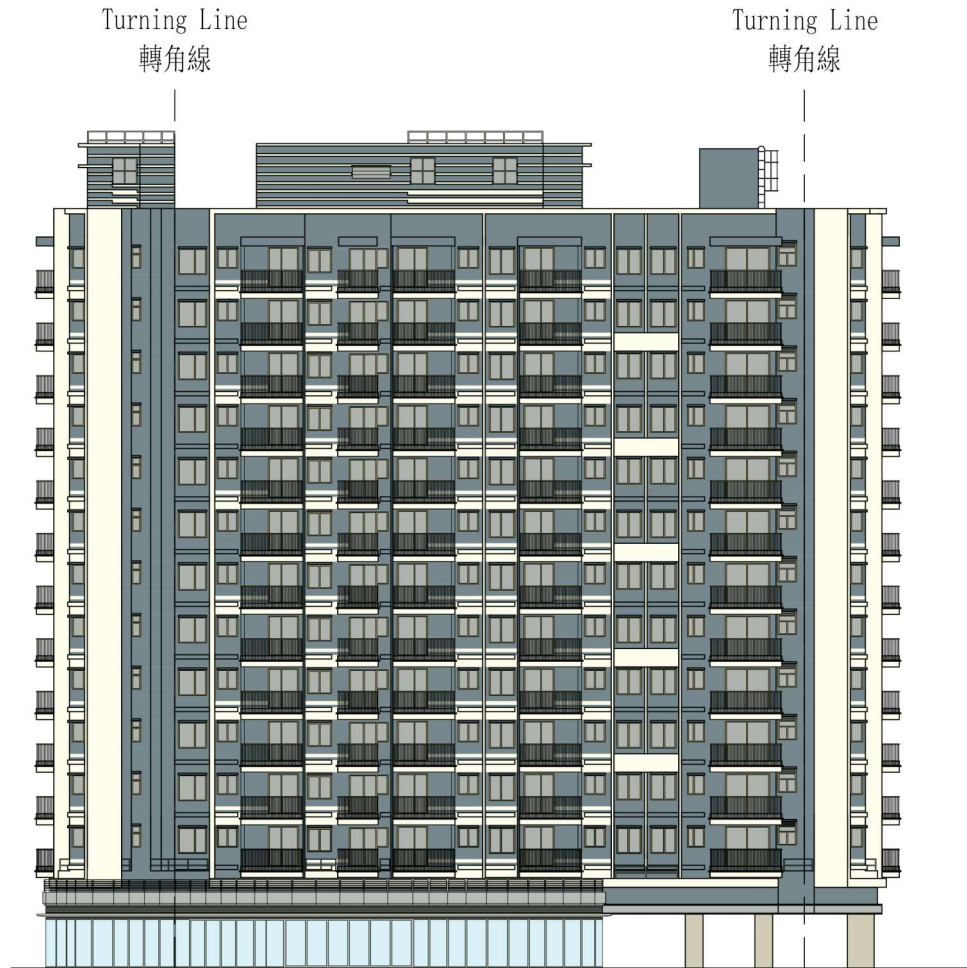
ELEVATION PLAN 4 立面圖4
