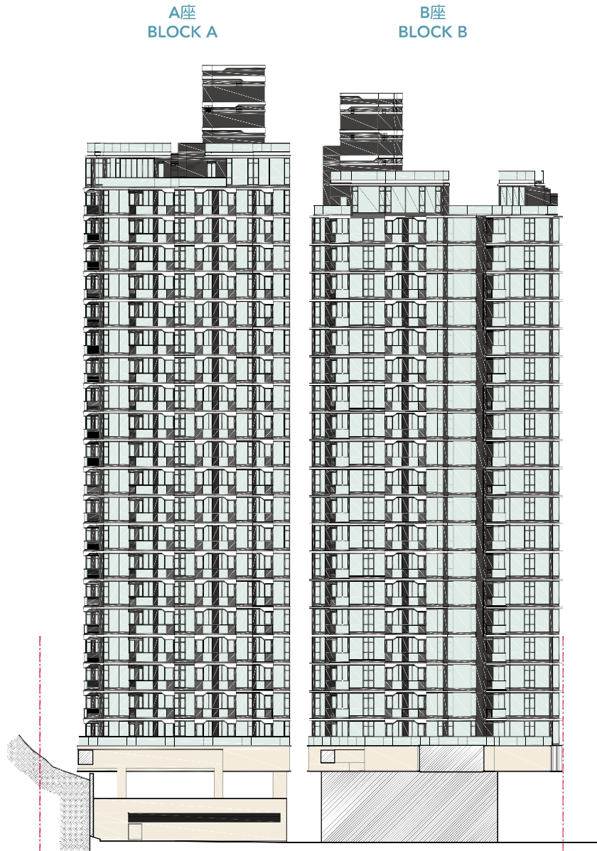
立面圖3 Elevation Plan 3
