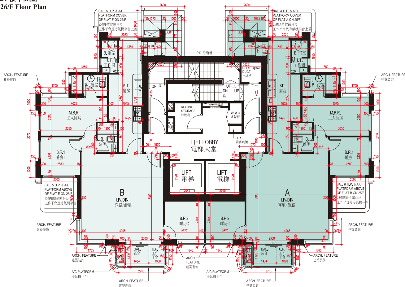
26 樓平面圖 26/F Floor Plan
