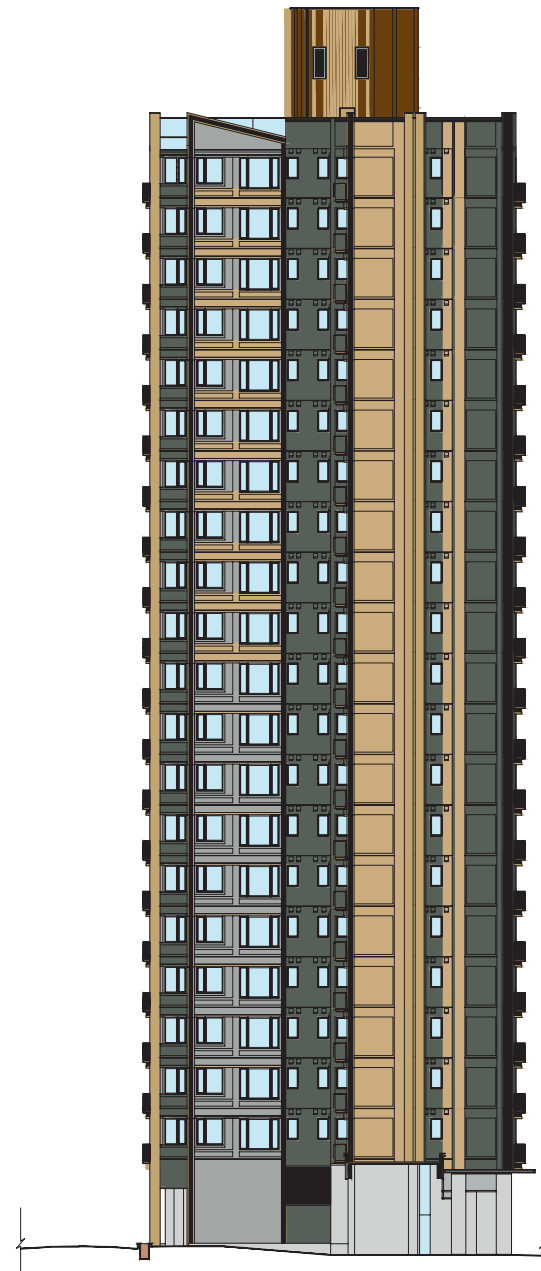
立面圖 C3 ELEVATION PLAN C3
