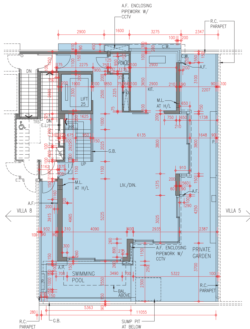
3/F Floor Plan 3樓樓面平面圖
