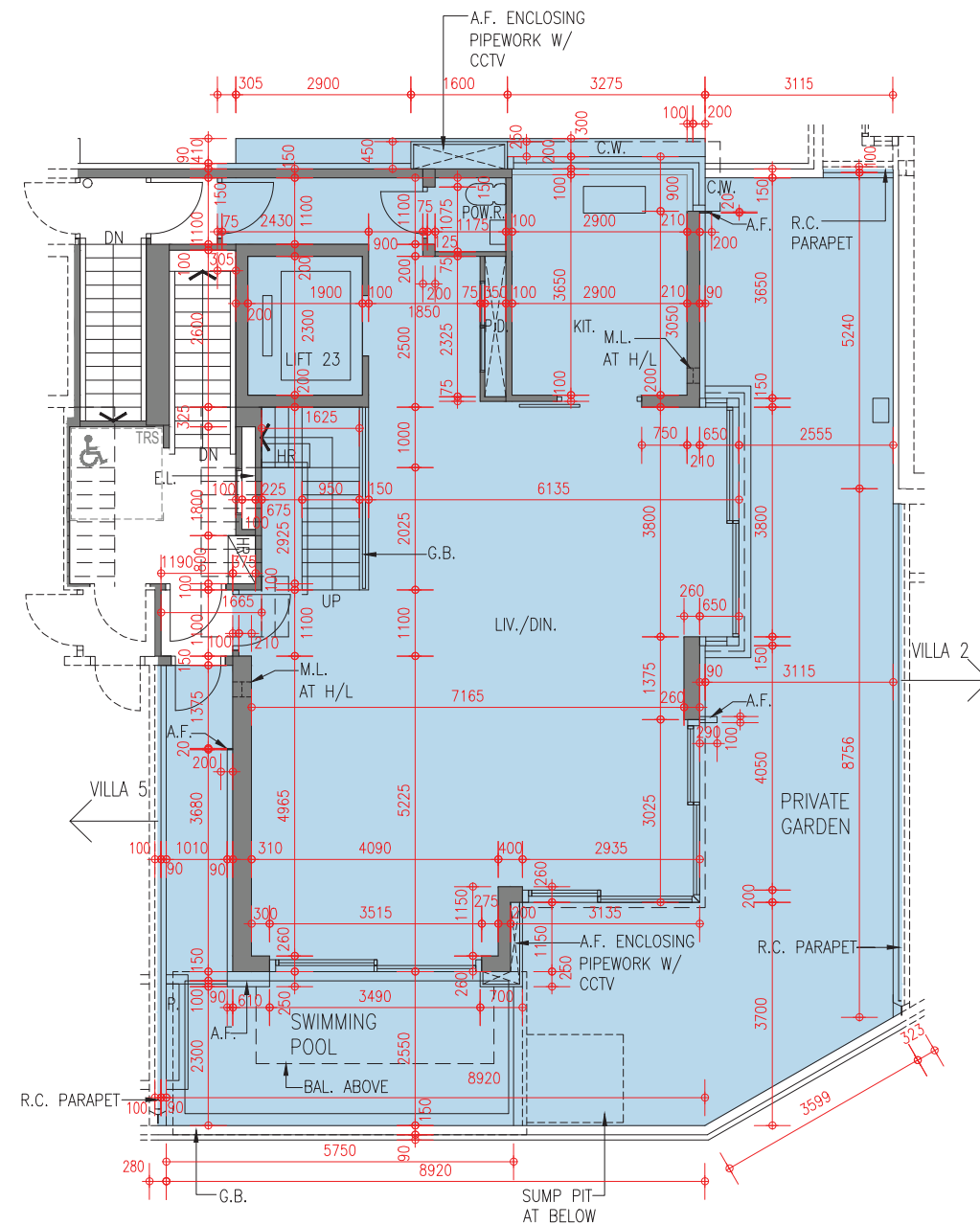
3/F Floor Plan 3樓樓面平面圖
