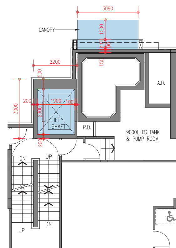
1/F Floor Plan
