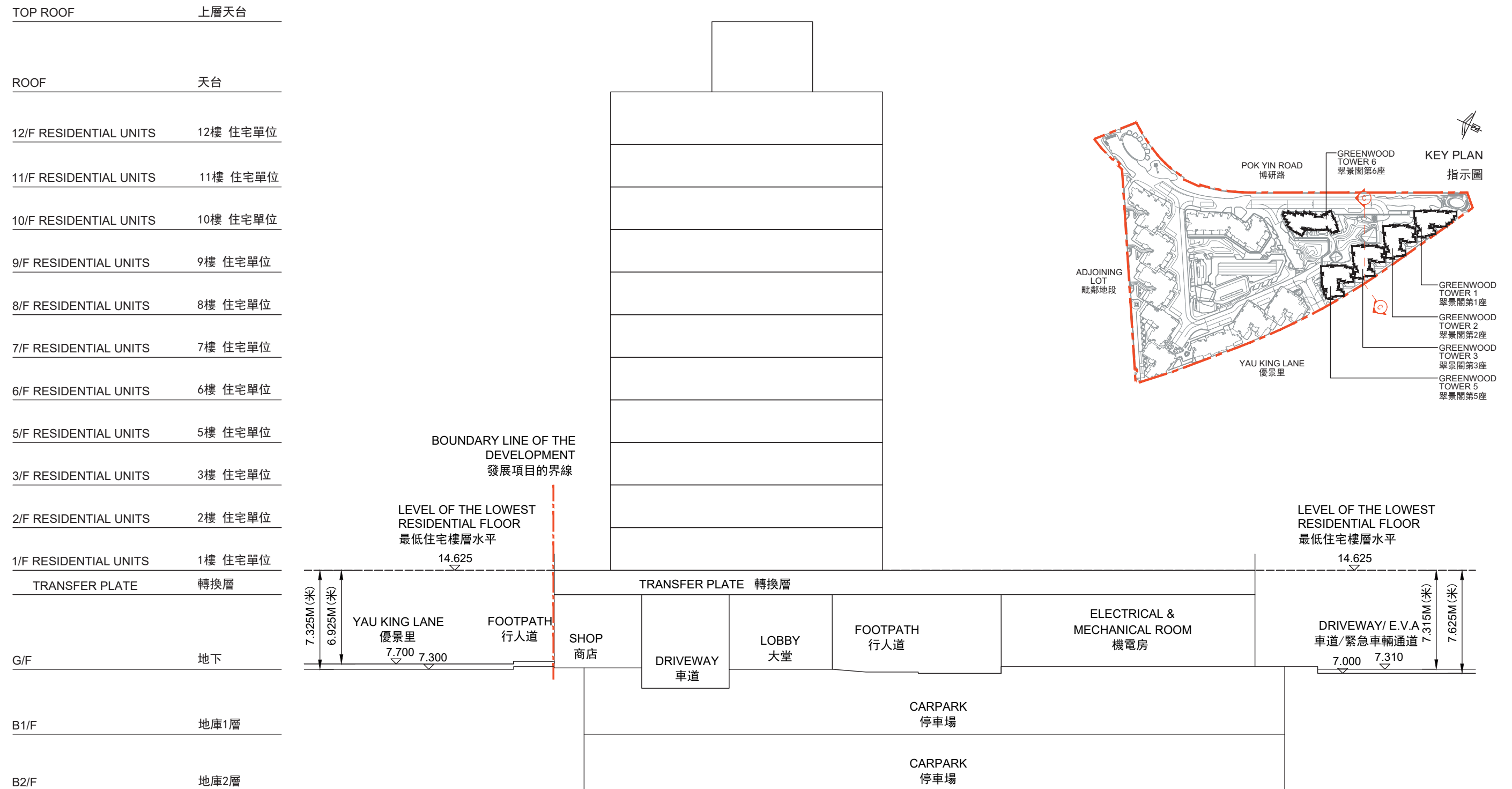
CROSS-SECTION PLAN C - C 橫截面圖 C - C
