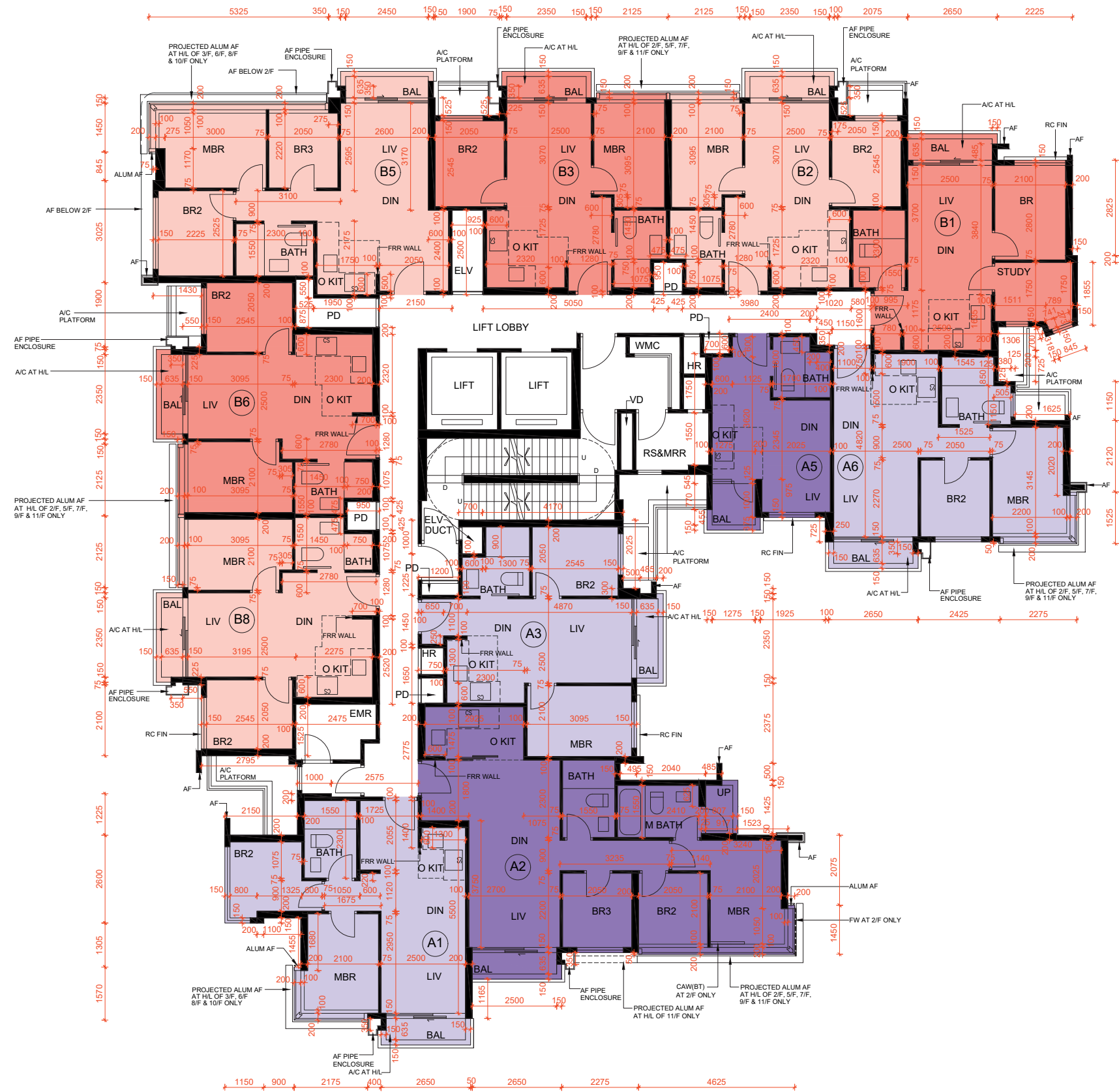
GREENWOOD TOWER 5 2/F-3/F AND 5/F-11/F FLOOR PLAN
