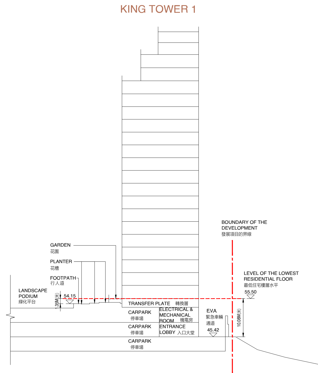
Cross-Section Plan A - A
