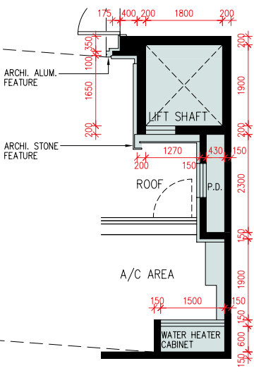
Roof Part Plan at Low Level 天台低位部分平面圖
