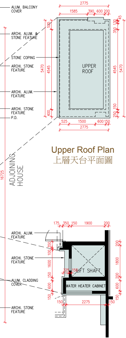
Roof Part Plan at Low Level 天台低位部分平面圖
