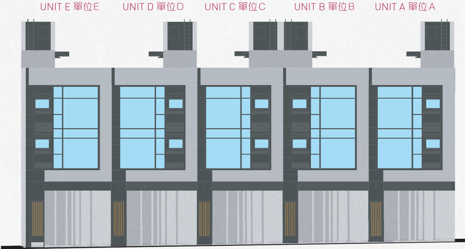
Elevation Plan 3 立面圖3
