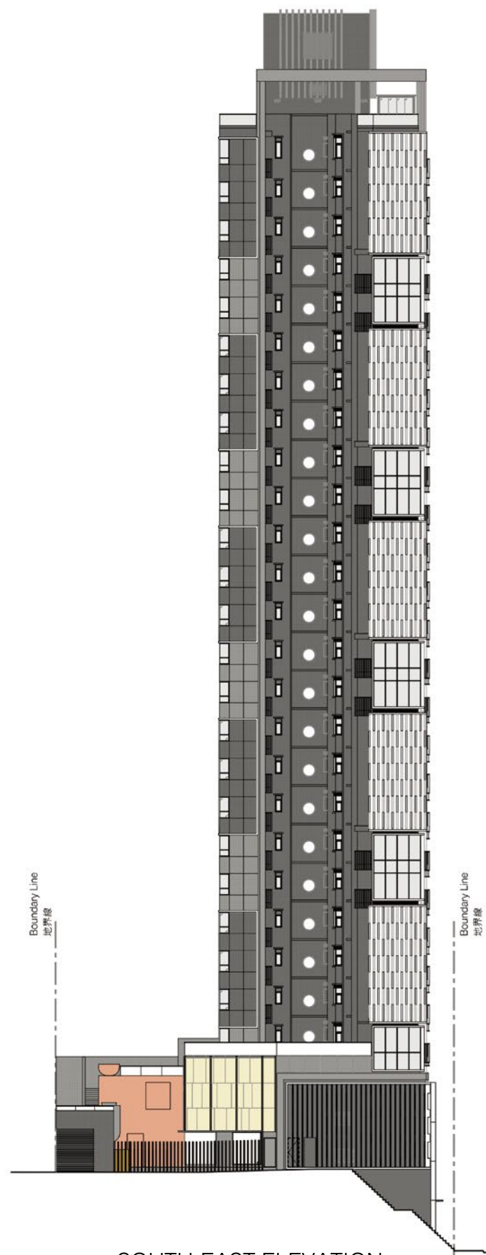
SOUTH-EAST ELEVATION 東南立面圖
