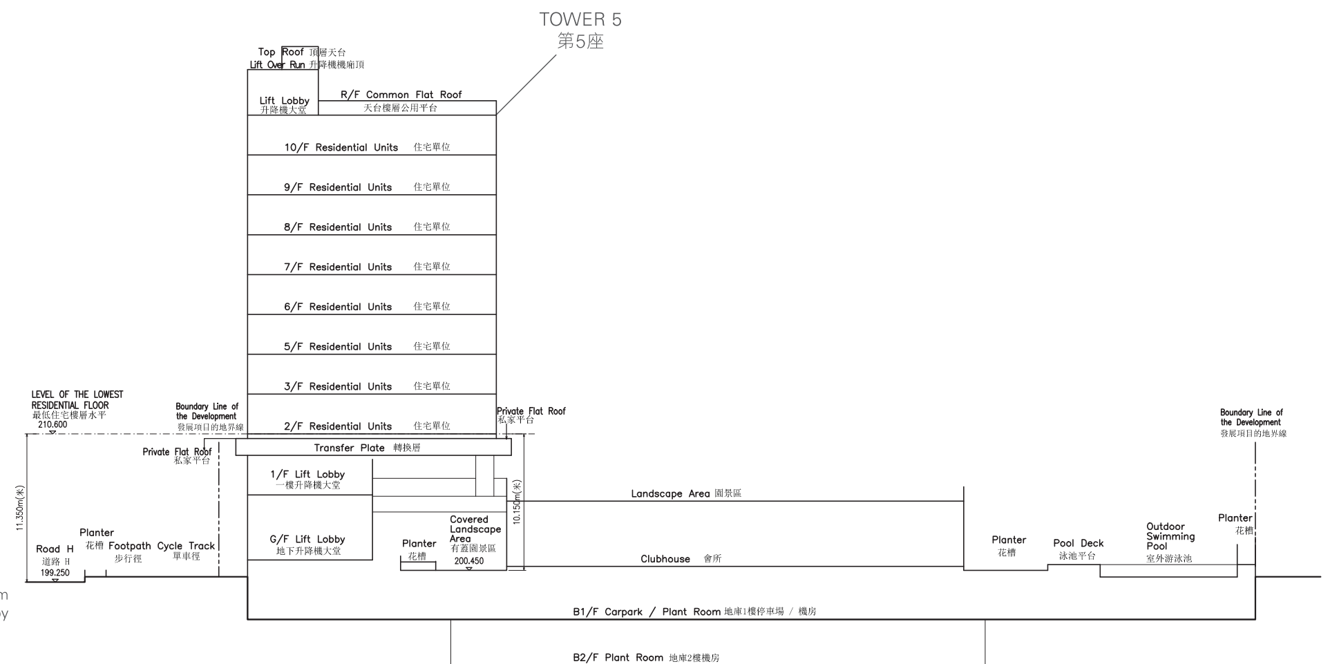
CROSS SECTION PLAN E 橫截面圖E
