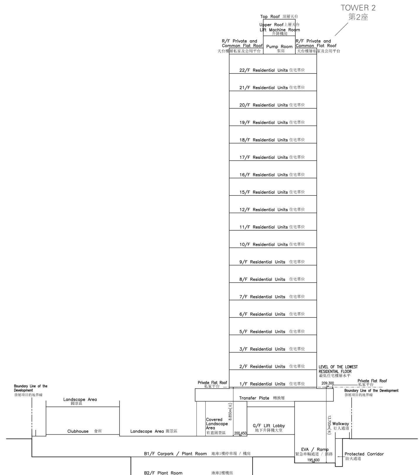
CROSS SECTION PLAN B 橫截面圖B
