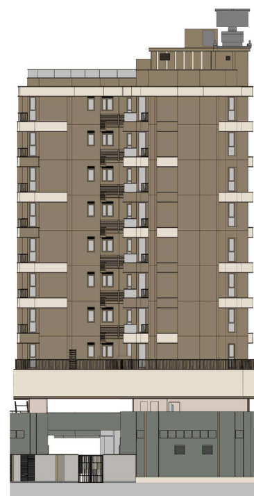
SOUTHWEST ELEVATION 西南面立面圖
