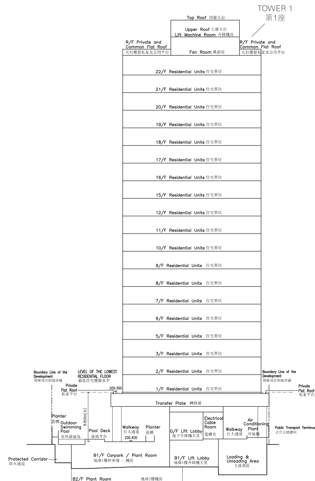
CROSS SECTION PLAN A 橫截面圖A
