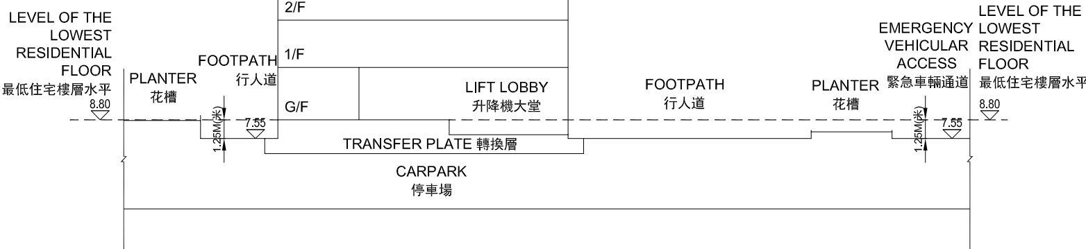
CROSS-SECTION PLAN C1 橫截面圖C1
