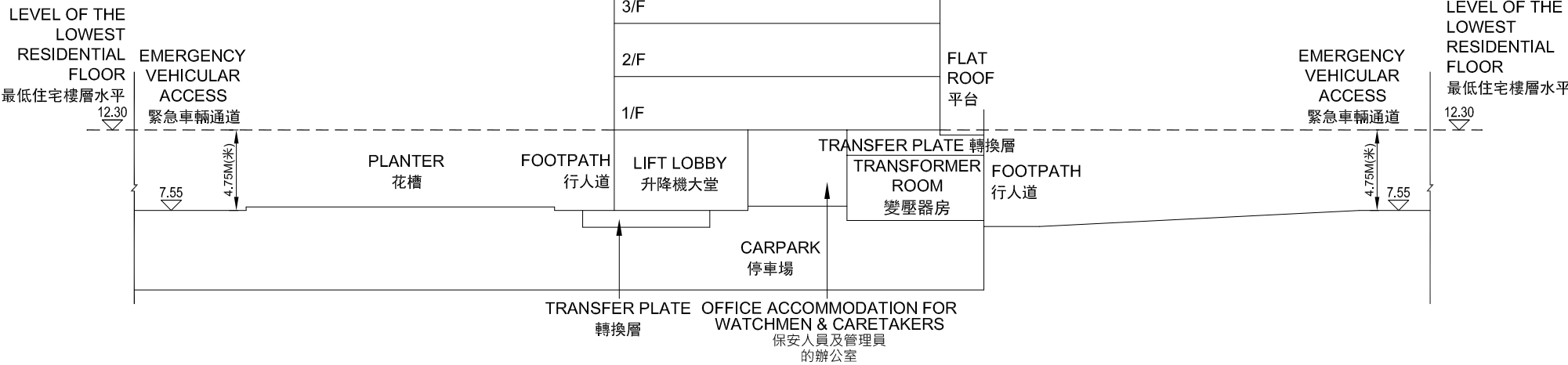
CROSS-SECTION PLAN B1 橫截面圖B1
