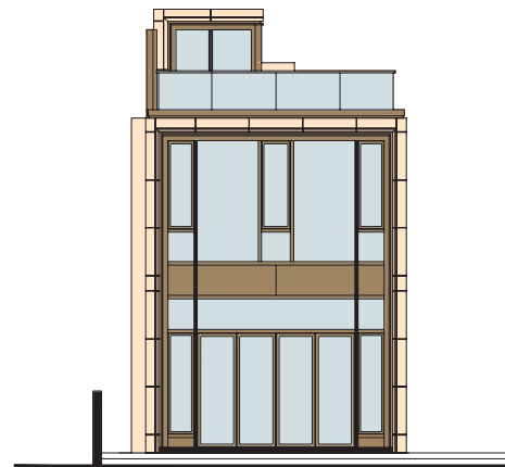
Elevation D (For House C1) 立面圖D (適用於C1號洋房)
