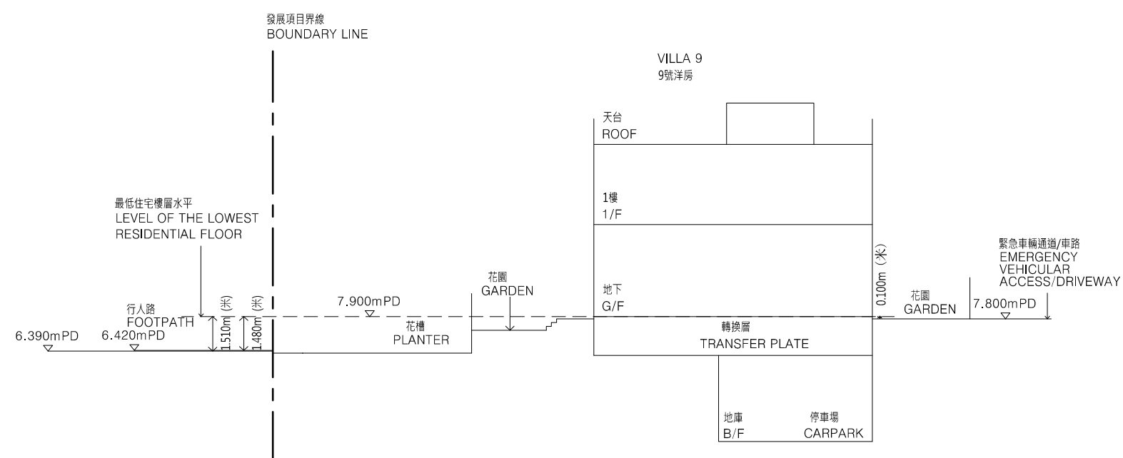
Cross Section Plan V9 橫截面圖V9
