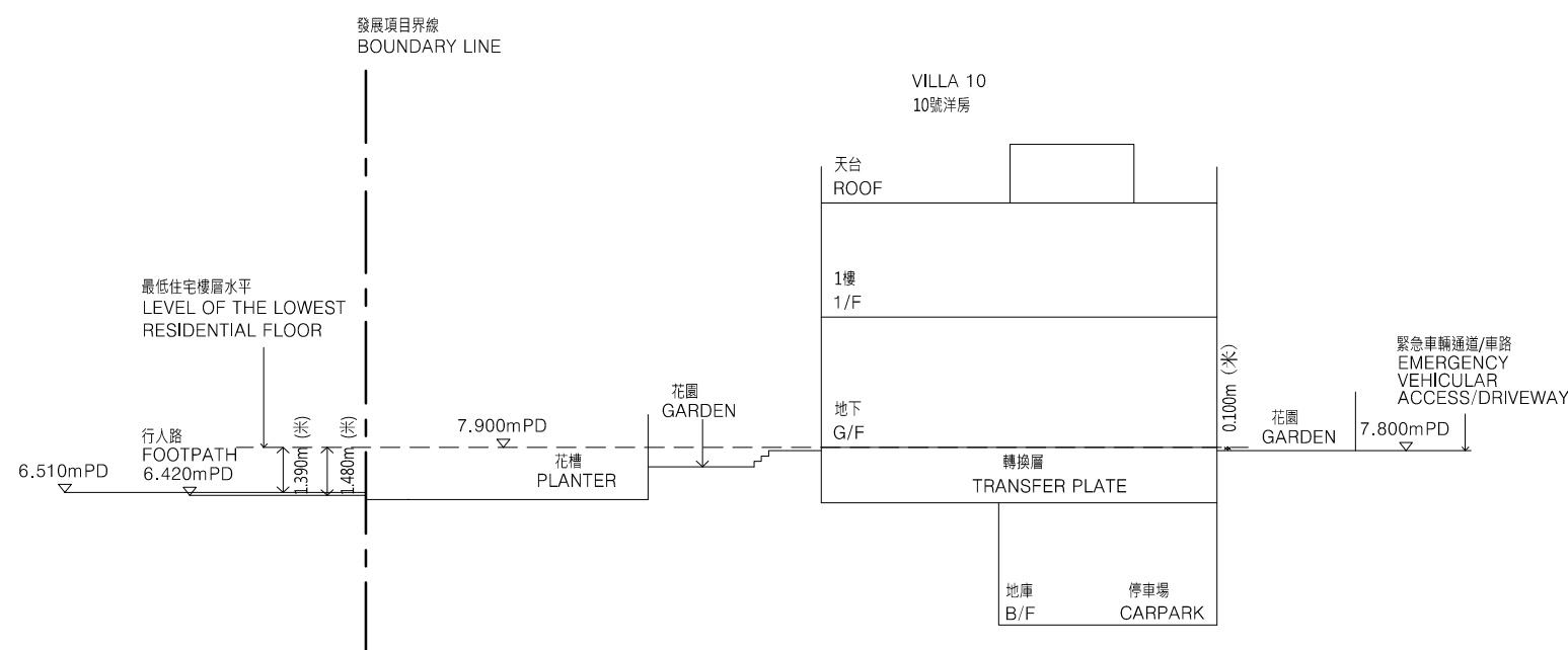
Cross Section Plan V10 橫截面圖V10
