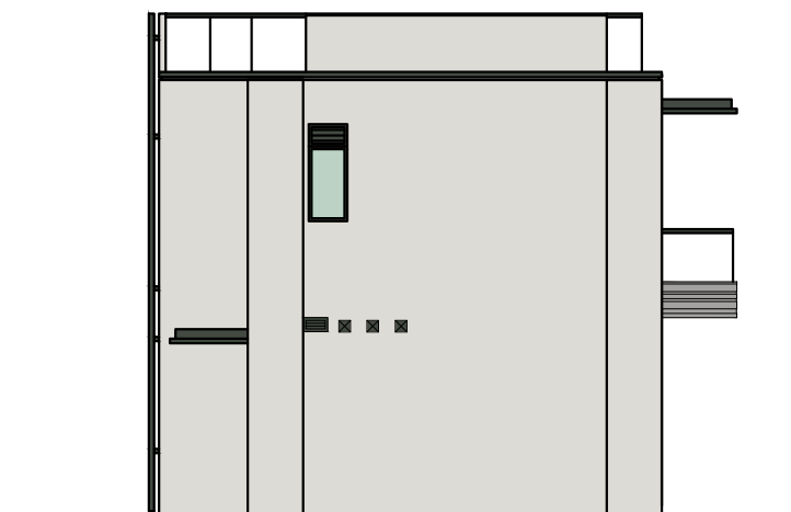
Elevation A (For Villa A) 立面圖A(適用於A號洋房)
