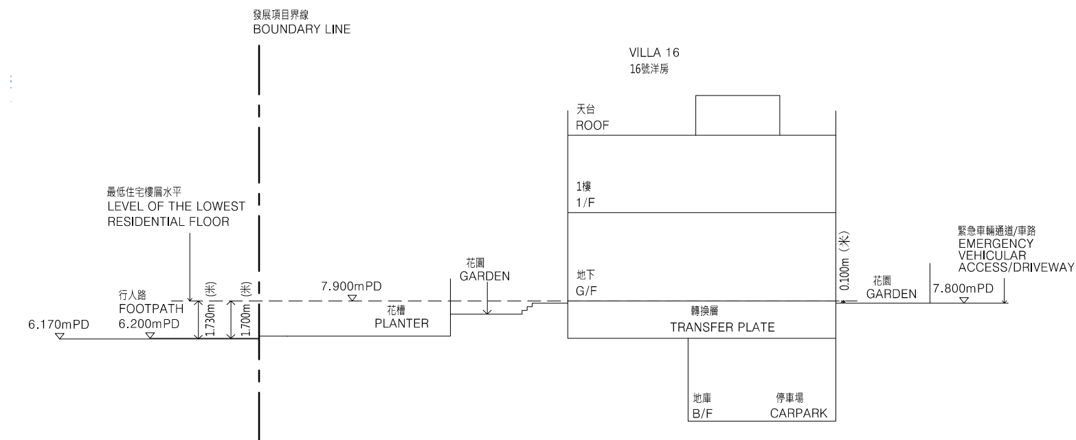
Cross Section Plan V16 橫截面圖V16
