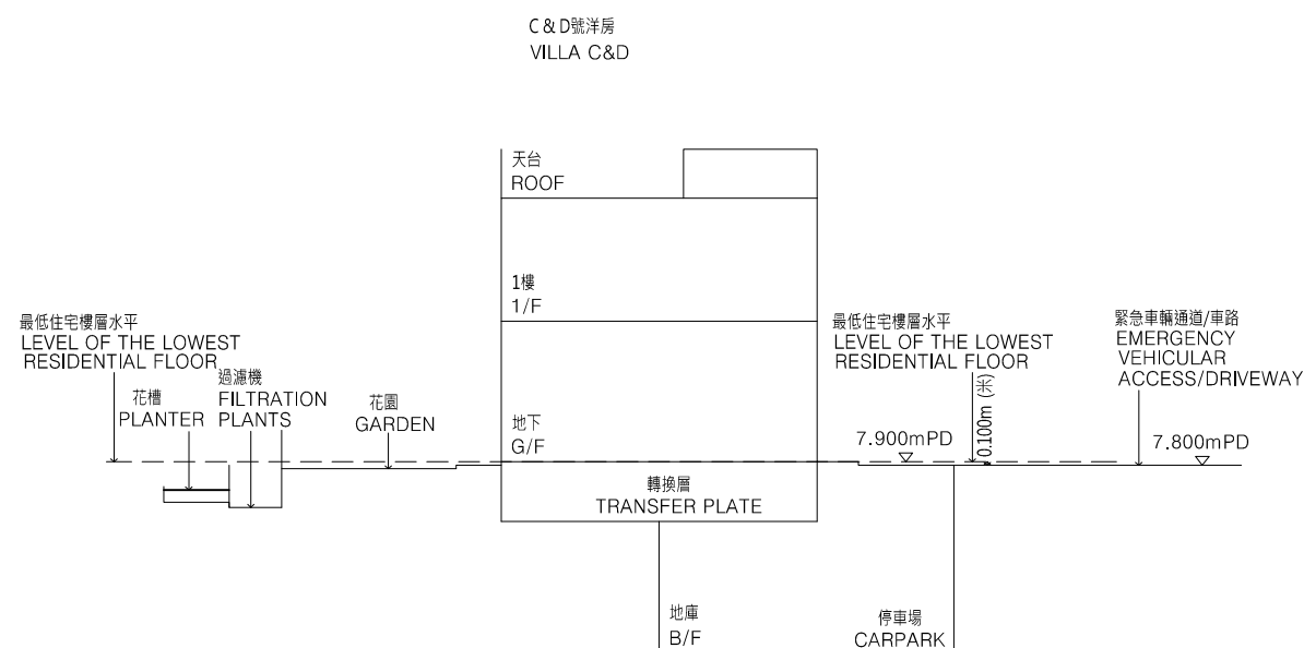
Cross Section Plan VB 橫截面圖VB
