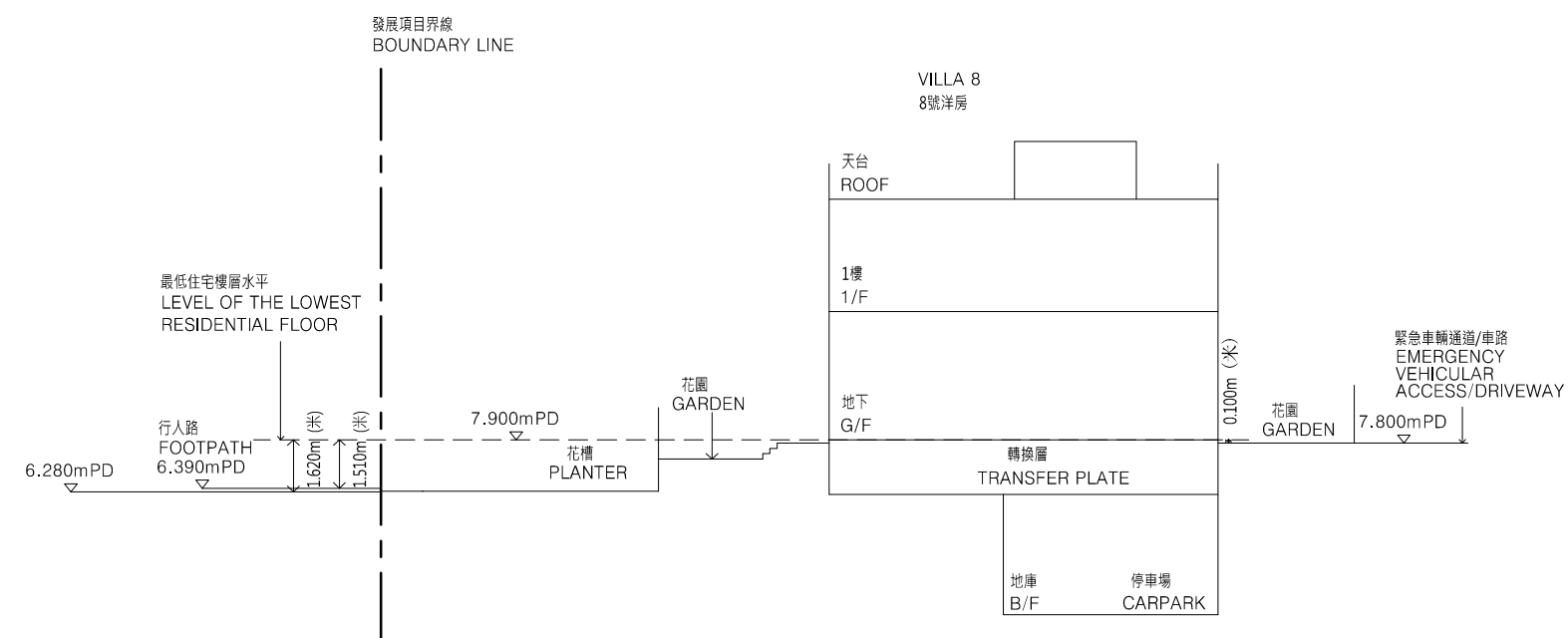
Cross Section Plan V8 橫截面圖V8
