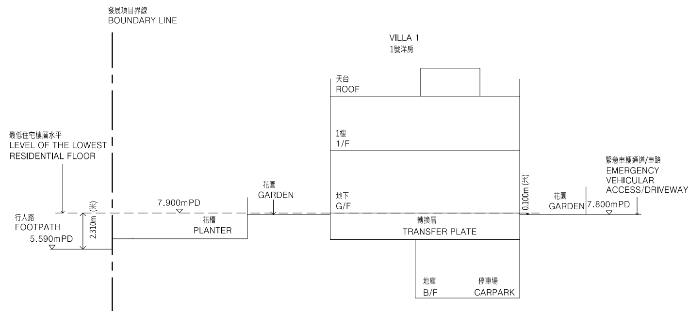
Cross Section Plan V1 橫截面圖V1
