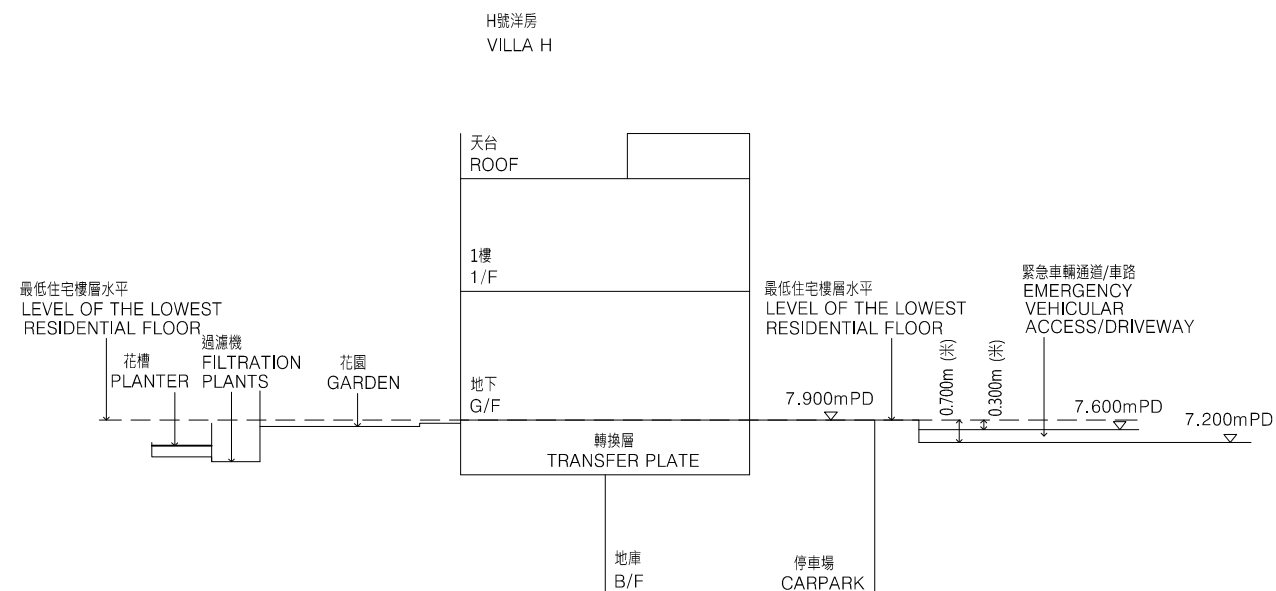
Cross Section Plan VC 橫截面圖VC
