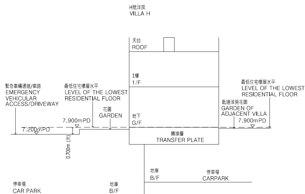
Cross Section Plan VD 橫截面圖VD
