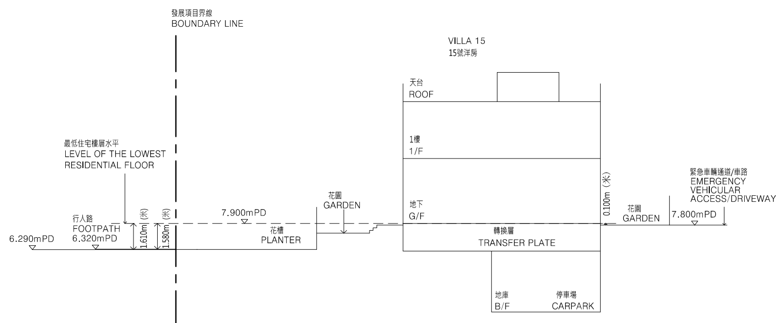
Cross Section Plan V15 橫截面圖V15
