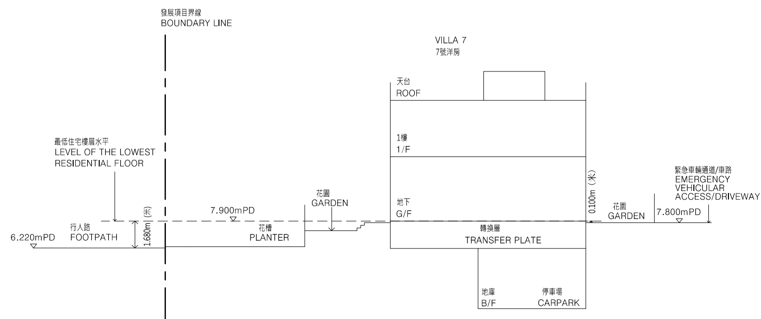
Cross Section Plan V7 橫截面圖V7
