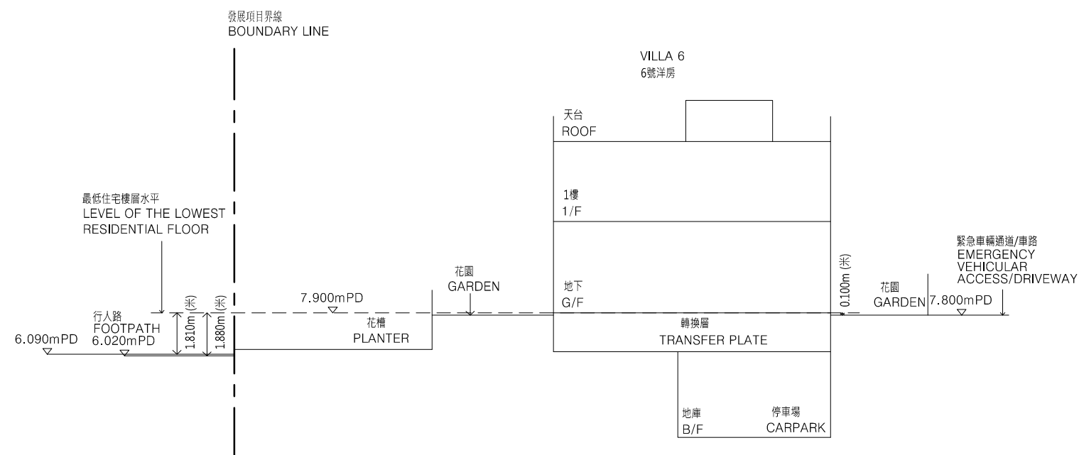
Cross Section Plan V6 橫截面圖V6
