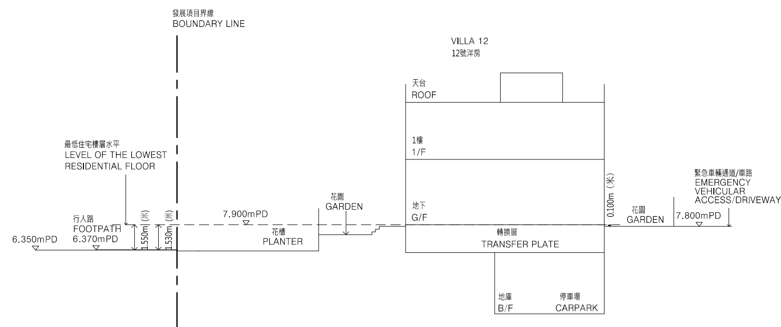
Cross Section Plan V12 橫截面圖V12
