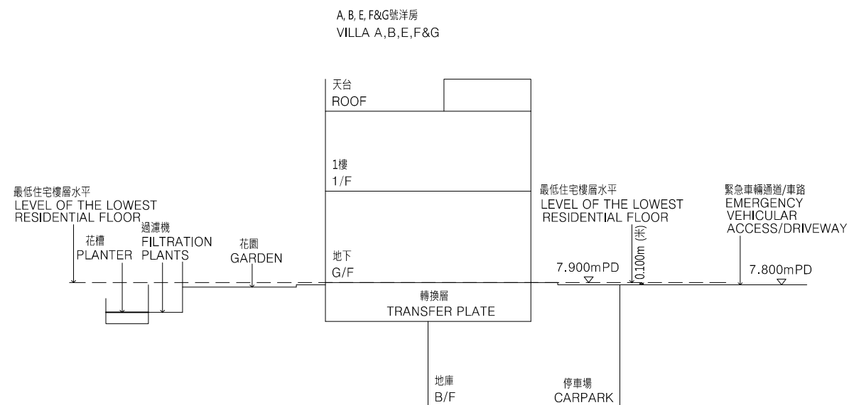
Cross Section Plan VA 橫截面圖VA
