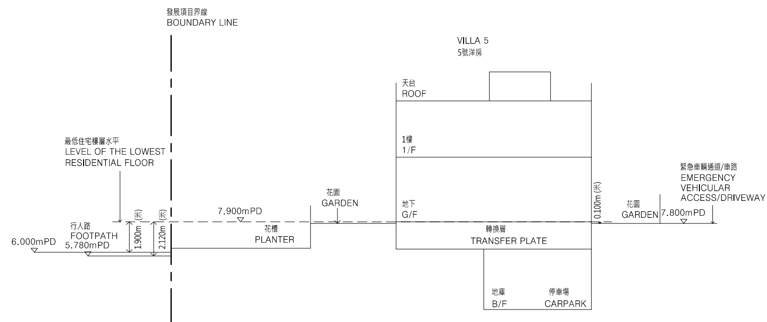
Cross Section Plan V5 橫截面圖V5
