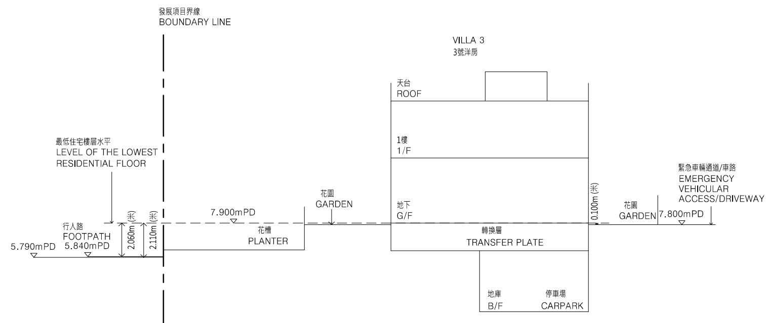
Cross Section Plan V3 橫截面圖V3
