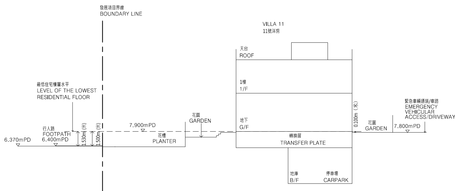
Cross Section Plan V11 橫截面圖V11
