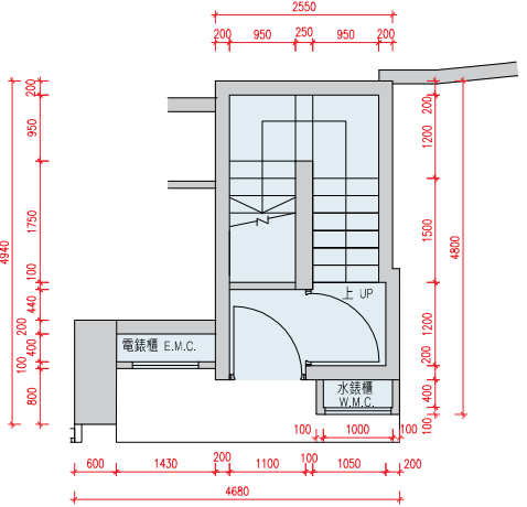
Part Plan of B/F Floor Plan 地庫局部平面圖
