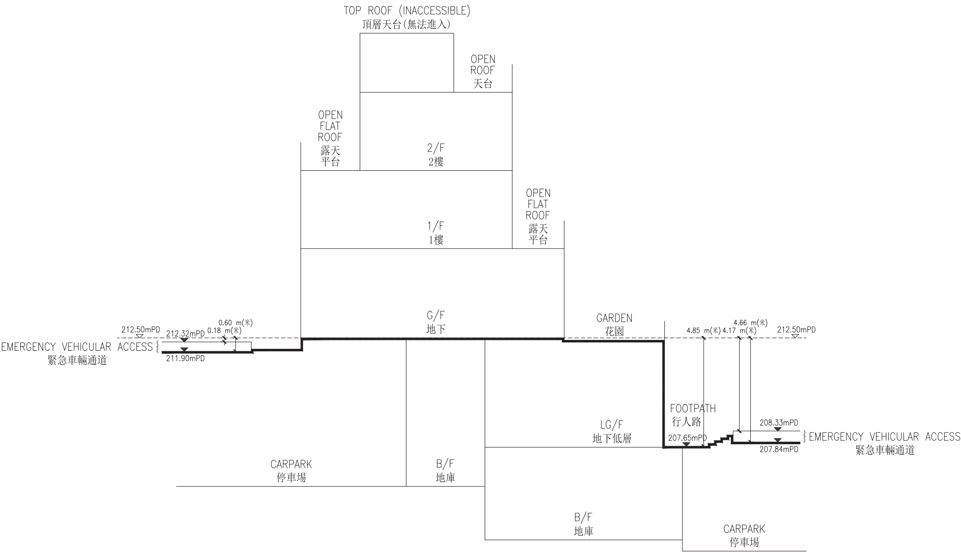
CROSS-SECTION PLAN H25 橫截面圖H25
