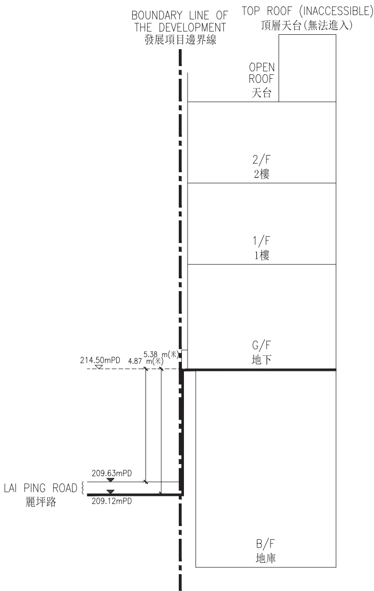
CROSS-SECTION PLAN H16B 橫截面圖H16B
