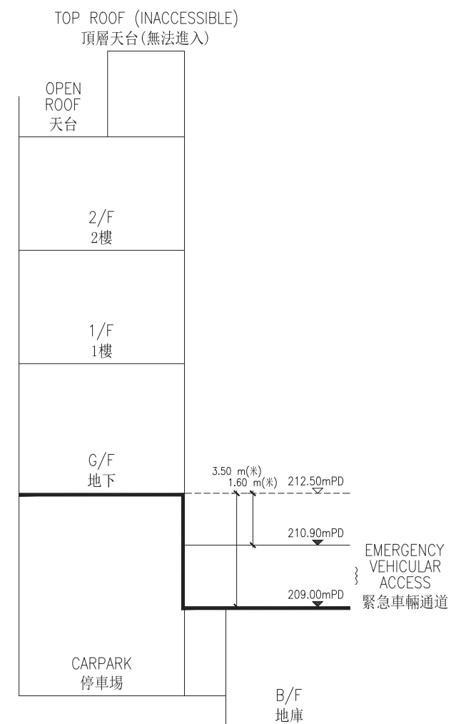
CROSS-SECTION PLAN H33B 橫截面圖H33B
