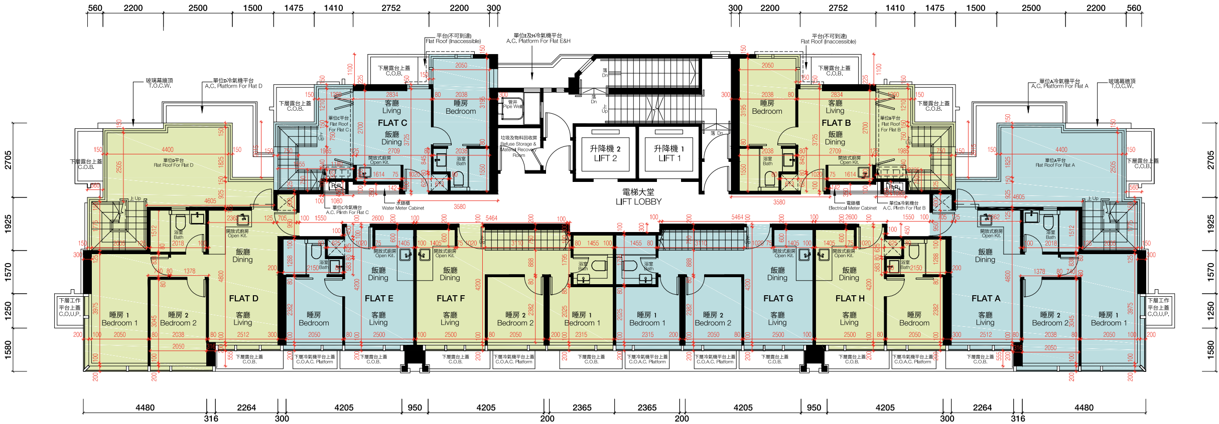
28樓平面圖 28th Floor Plan
