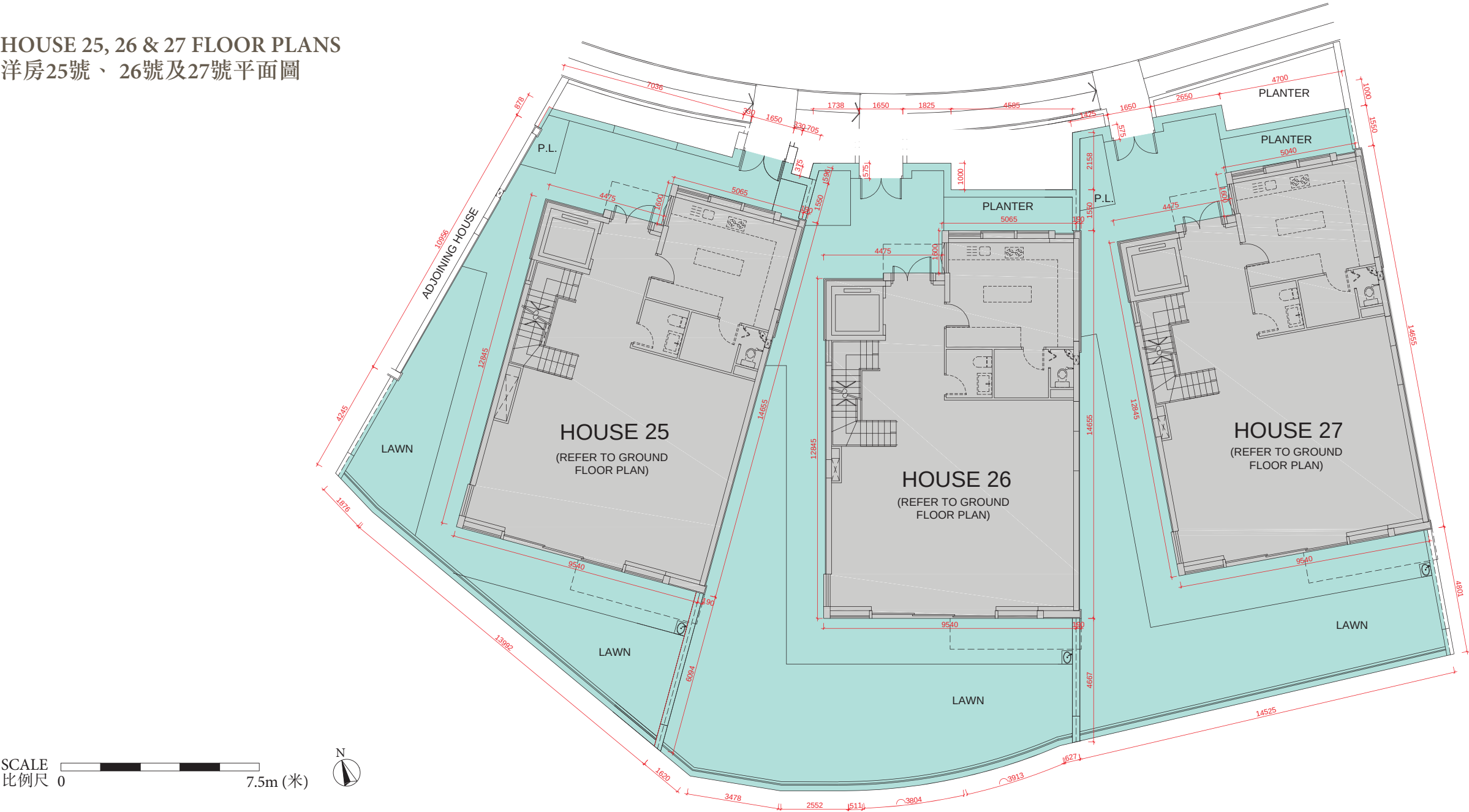
G/F PLAN (FOR GARDEN AREA ONLY) 地面層平面圖 (花園)
