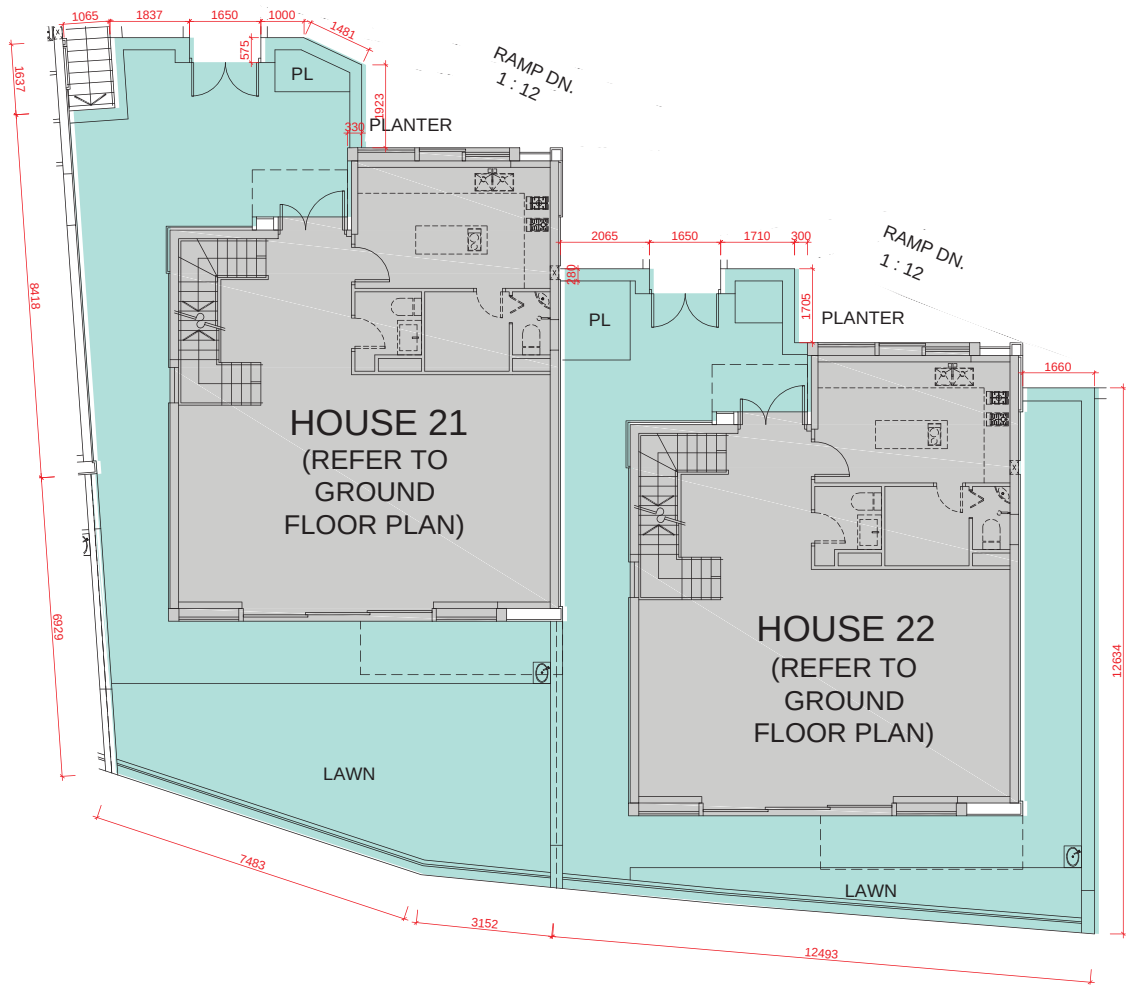
G/F PLAN (FOR GARDEN AREA ONLY) 地面層平面圖 (花園)
