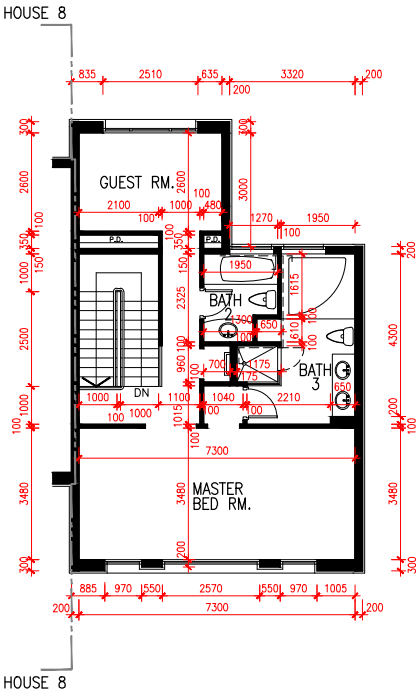
2/F PLAN
