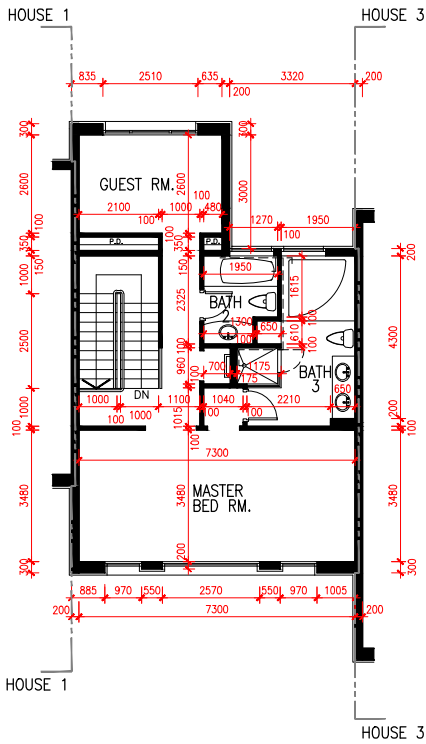
2/F PLAN
