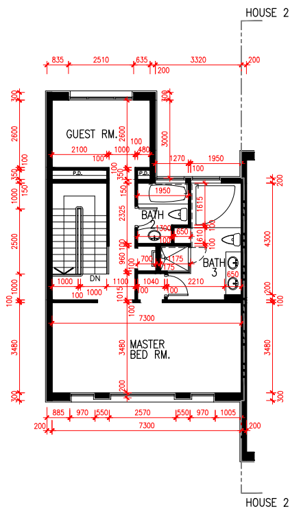
2/F PLAN
