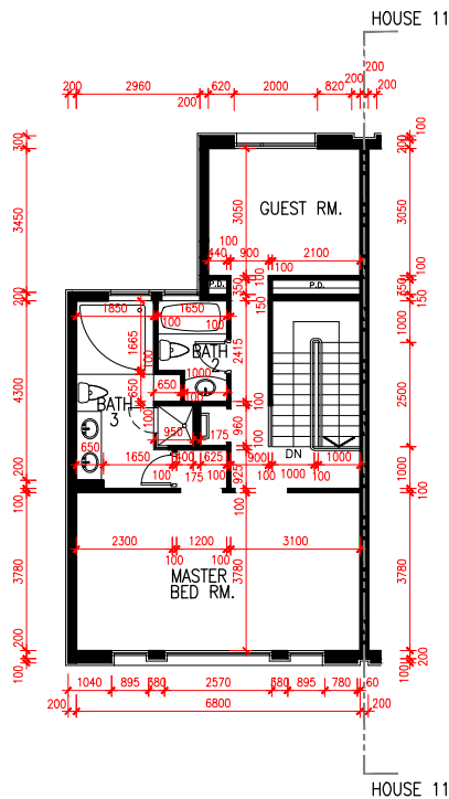
2/F PLAN
