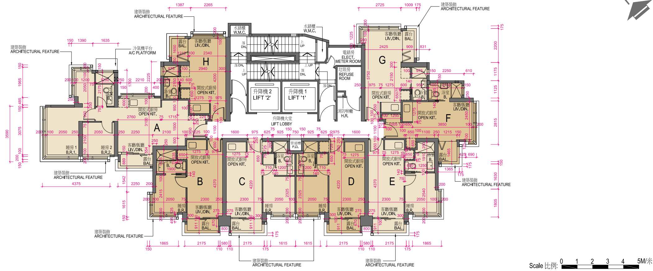
5樓、7樓及9樓平面圖 5th, 7th & 9th FLOOR PLAN
