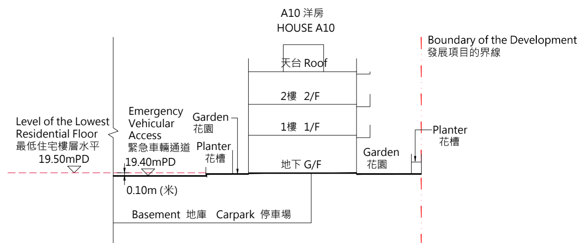
Cross-section Plan A10 橫截面圖 A10
