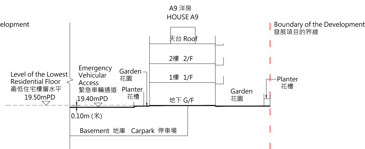
Cross-section Plan A9 橫截面圖 A9
