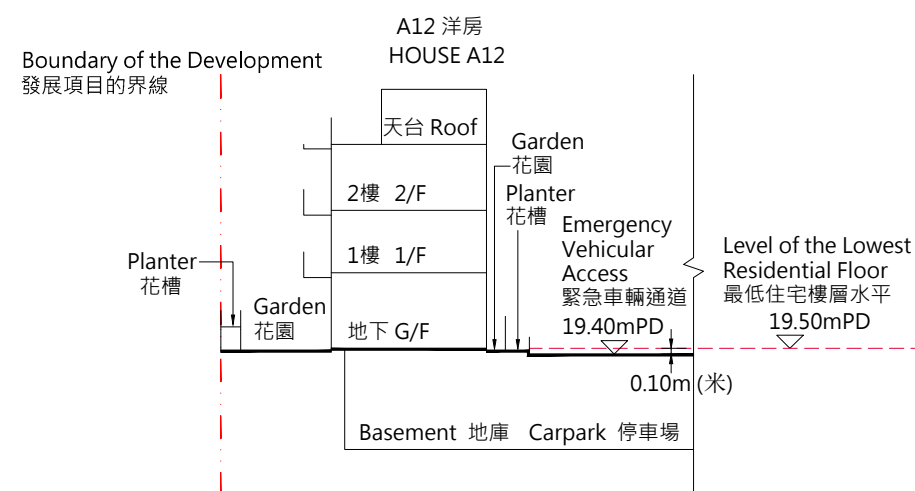
Cross-section Plan A12 橫截面圖 A12
