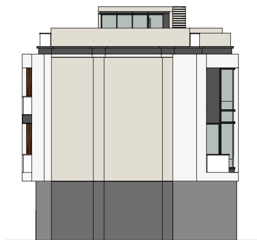
立面圖 C (適用於 B2, B5, B7, B8, B10, B12, A5, A7 和 A9 洋房) Elevation Plan C (For Houses B2, B5, B7, B8, B10, B12, A5, A7 & A9)
