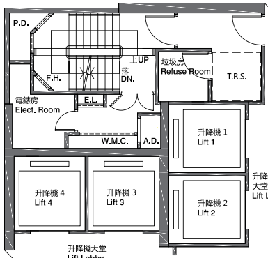
11樓及16樓之部分平面圖 PART PLAN FOR 11/F AND 16/F ONLY
